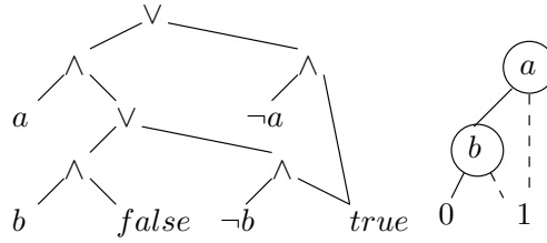
Figure 3. On the left part, a formula in the \text{OBDD}_{<} language. On the right part, a more standard notation for it.
