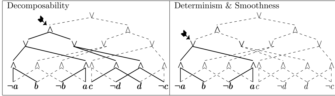
Figure 2. A formula in \text{NNF}_{PS} . On the left part, the node marked \clubsuit is decomposable while the node marked with the same symbol on the right part denotes a deterministic and smooth node.
