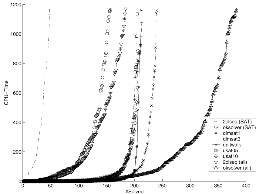
Figure 3. Number of instances solved vs. CPU time for SOTA contributors: Randomly generated benchmarks (note that the CPU time slice was smaller for these benchmarks). For each complete solvers (2c1seq and oksolver), we plot two curves: (1) a curve for SAT results only (in order to compare their performances to uncomplete solvers) and (2) for all benchmarks (SAT+UNSAT).
